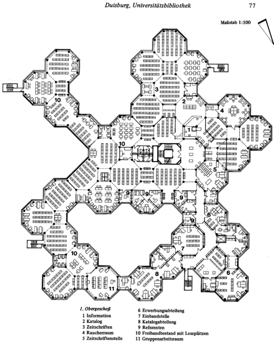
Diagram 9: University of Duisburg floor plan.
