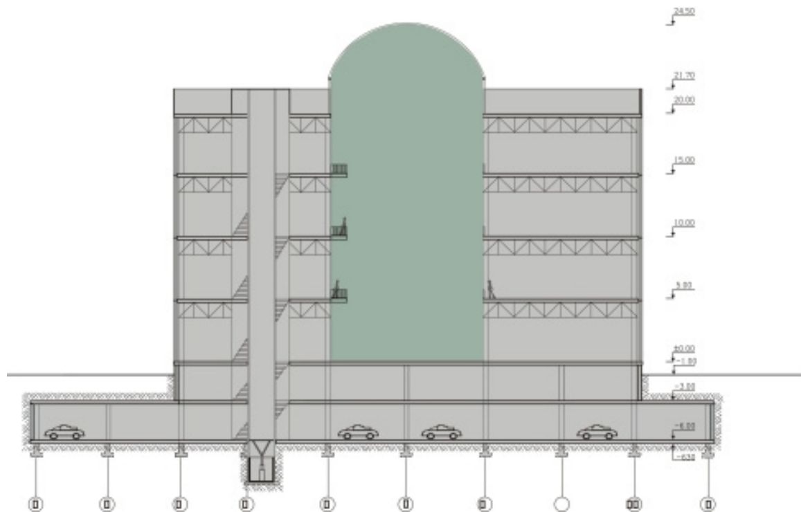
Fig. 4. Cross – section of the building
